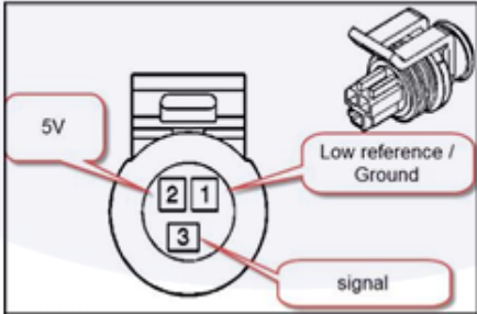
View looking into connector.
